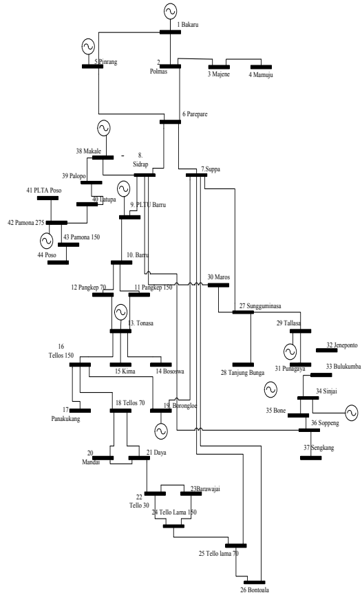
Fig.1 Single line diagram of Sulselbar transmission system
